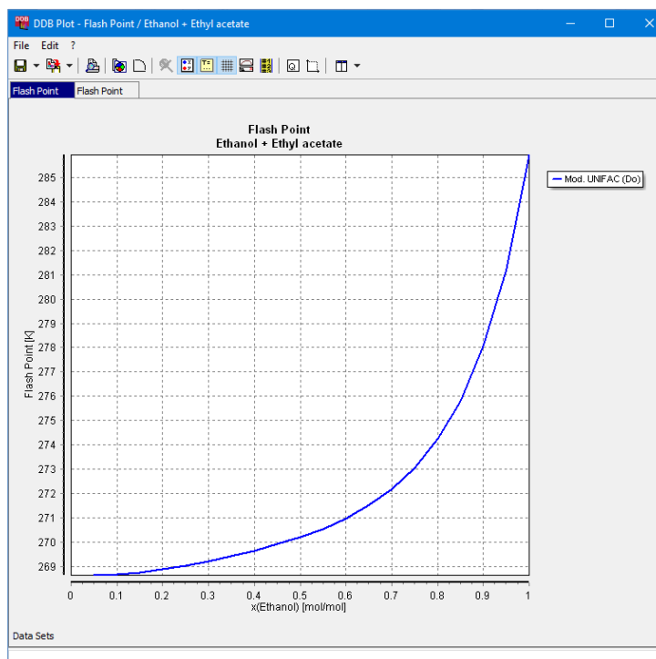
Figure 3: Flashpoint diagram of a binary mixture.
