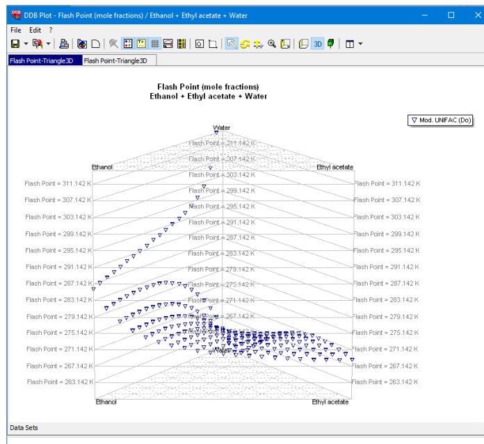
Figure 2: Flashpoint diagram of a ternary mixture.
