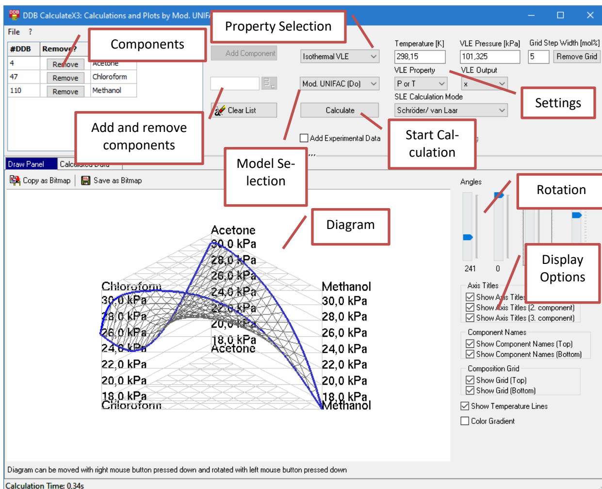
Figure 1: Main window.
