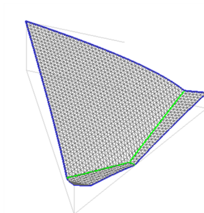
Figure 6: m -xylene – p -xylene - tetrachloromethane
