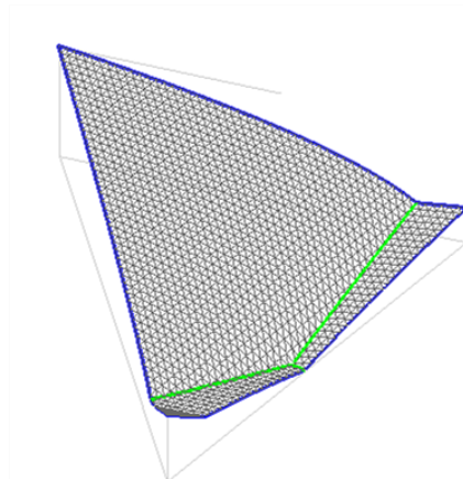
Figure 6: m -xylene – p -xylene - tetrachloromethane
