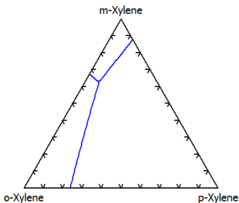
Figure 7: Eutectic lines.
