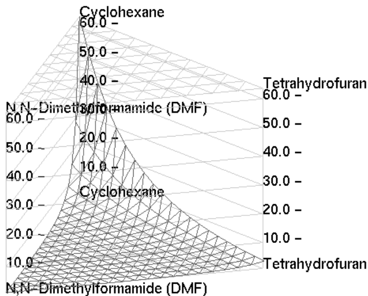
Figure 13: System DMF – THF – cyclohexane.
