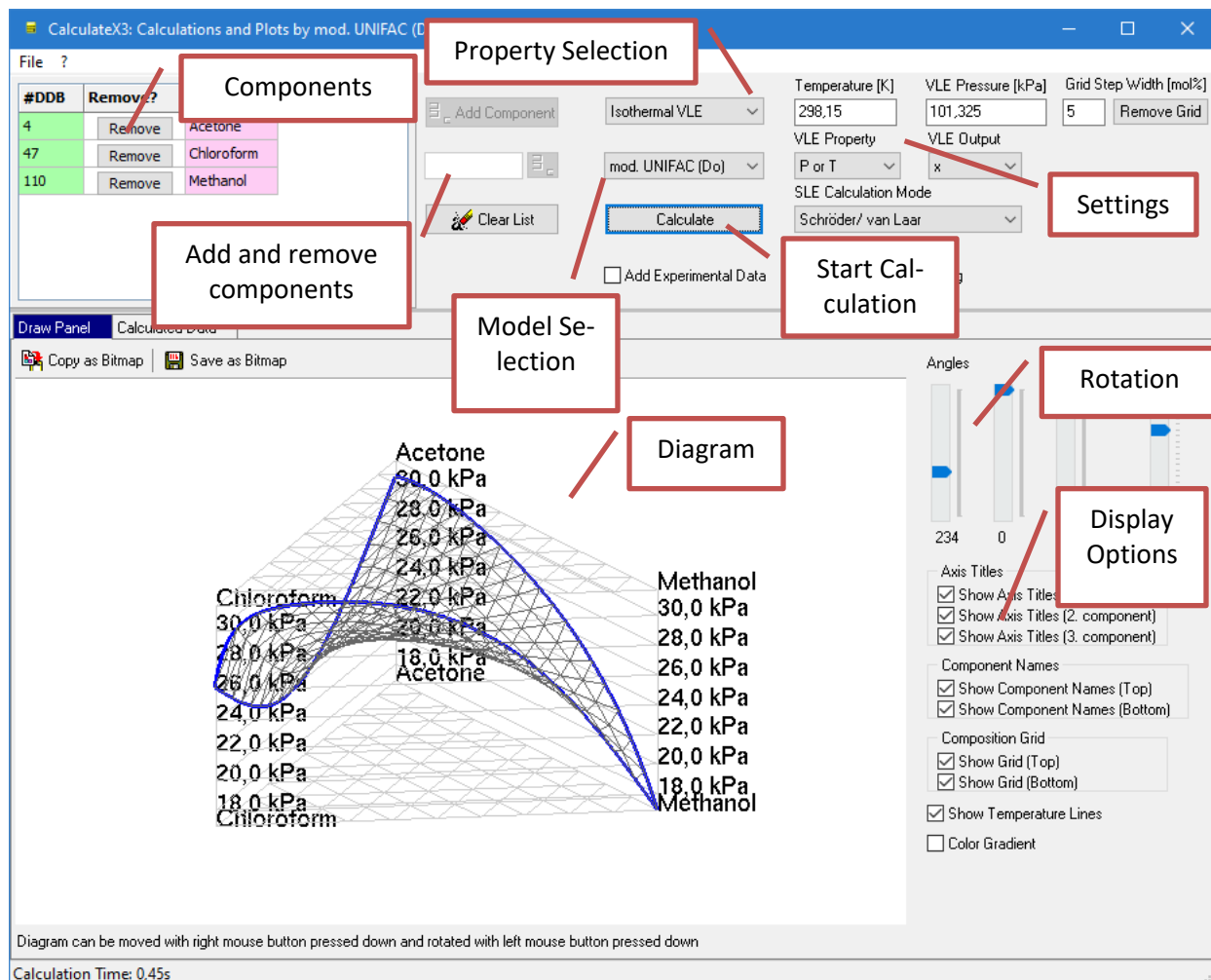
Figure 1: Main window.
