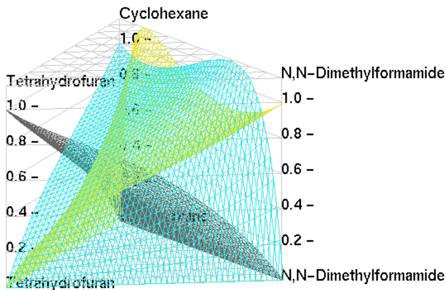
Figure 15: Activities for the ternary system DMS – THF – cyclohexane.
