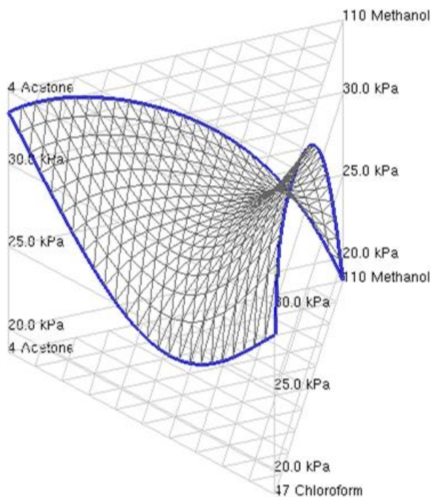
Figure 8: Methanol – acetone - chloroform
