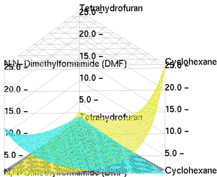
Figure 14: Activity coefficients for the ternary system DMF – THF – cyclohexane.
