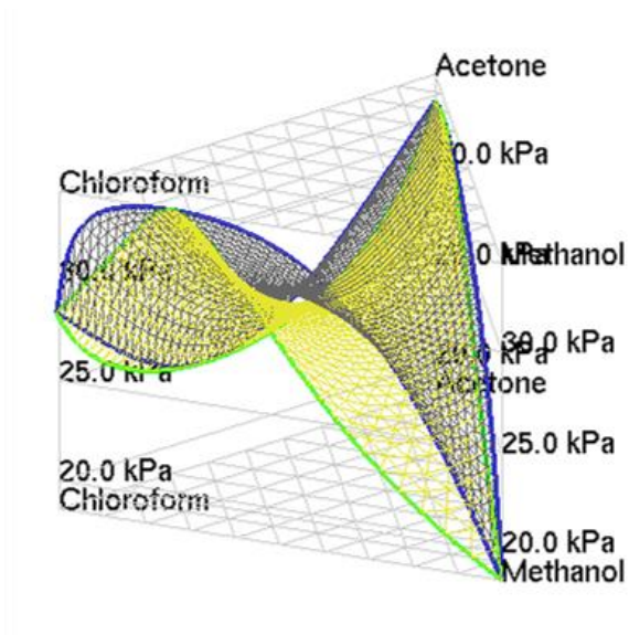
Figure 10: Vapor and liquid composition planes.
